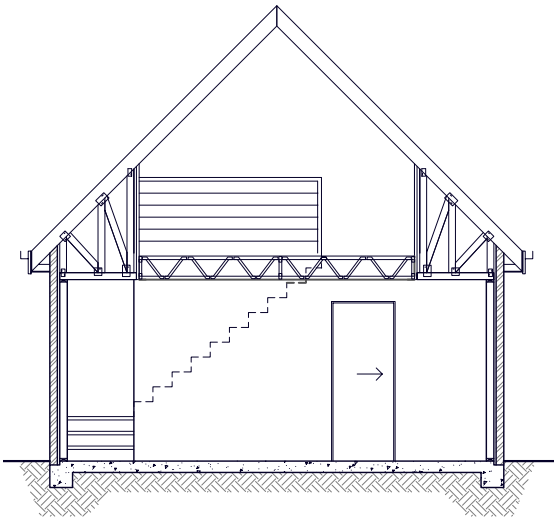
SECTION 1:100
