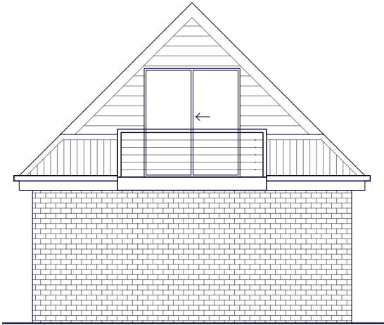
FRONT ELEVATION 1:100
